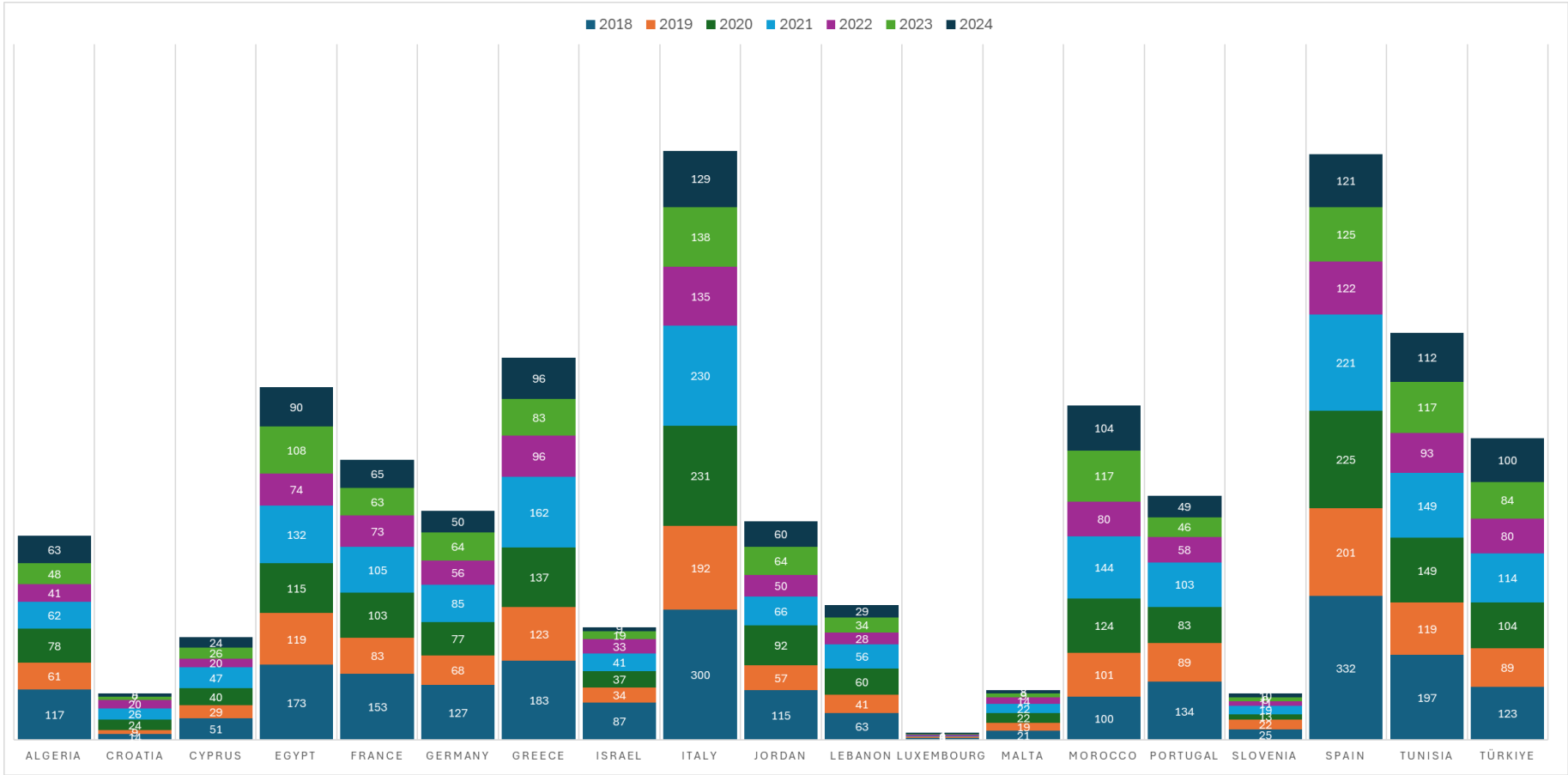
Figure 6 Section 1: Number of Submitted proposals per Participating State per year (2018- 2024)
