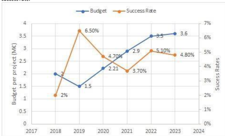
Figure 1: Trends in budget per project (in million euros, M€) and success rate (%) from 2018 to 2023. The blue line represents the average budget per project per year, while the orange line indicates the success rate.
