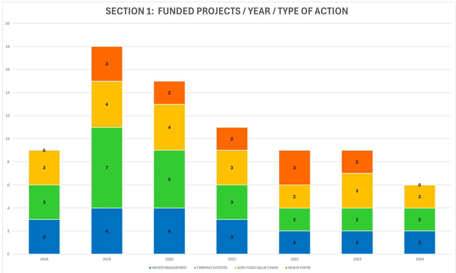
Figure 29 Section 1 Funded projects per thematic area 2018- 2024
